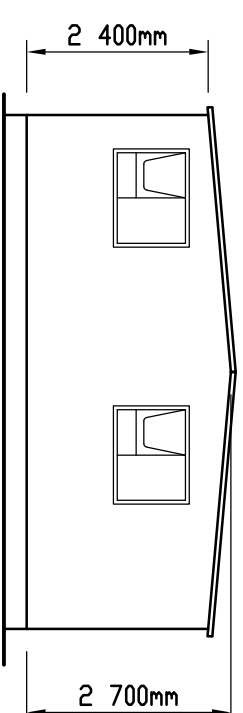
LEFT ELEVATION
