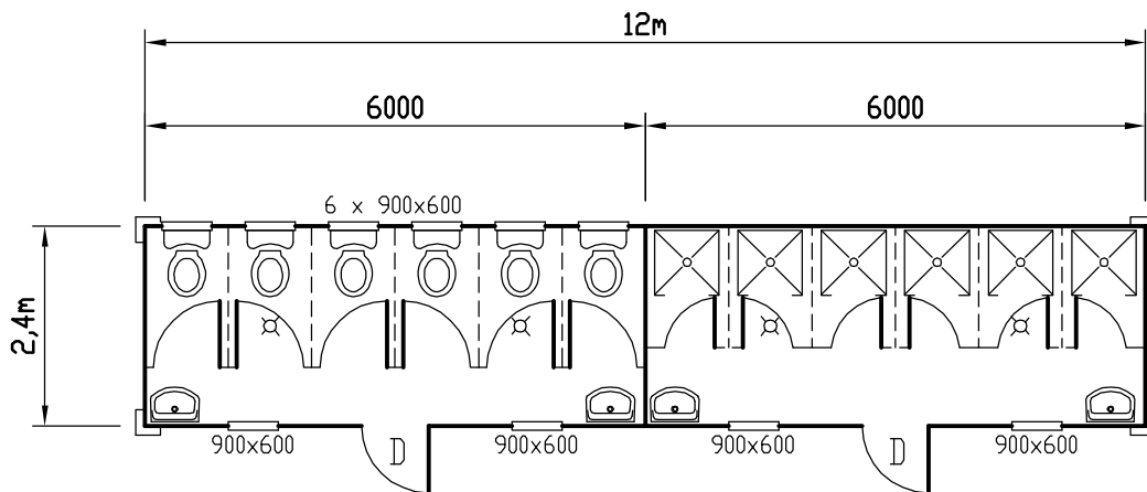
PLAN 28,8m 2
