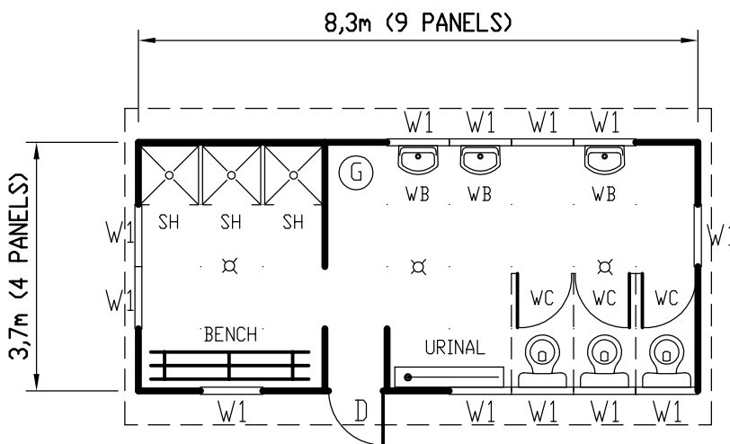
PLAN 31m 2
