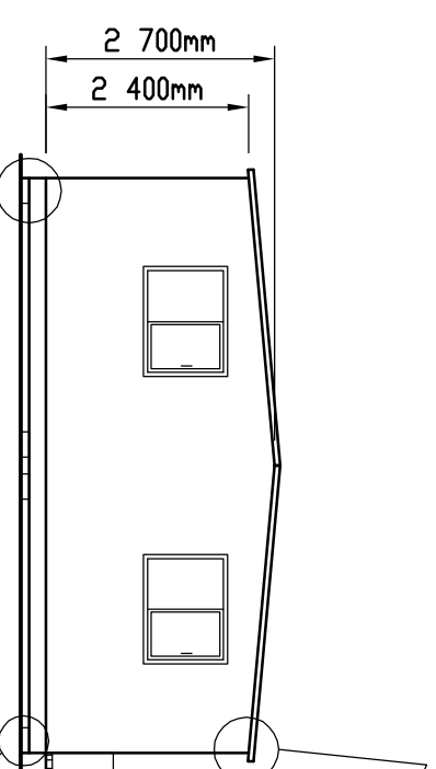
LEFT ELEVATION
