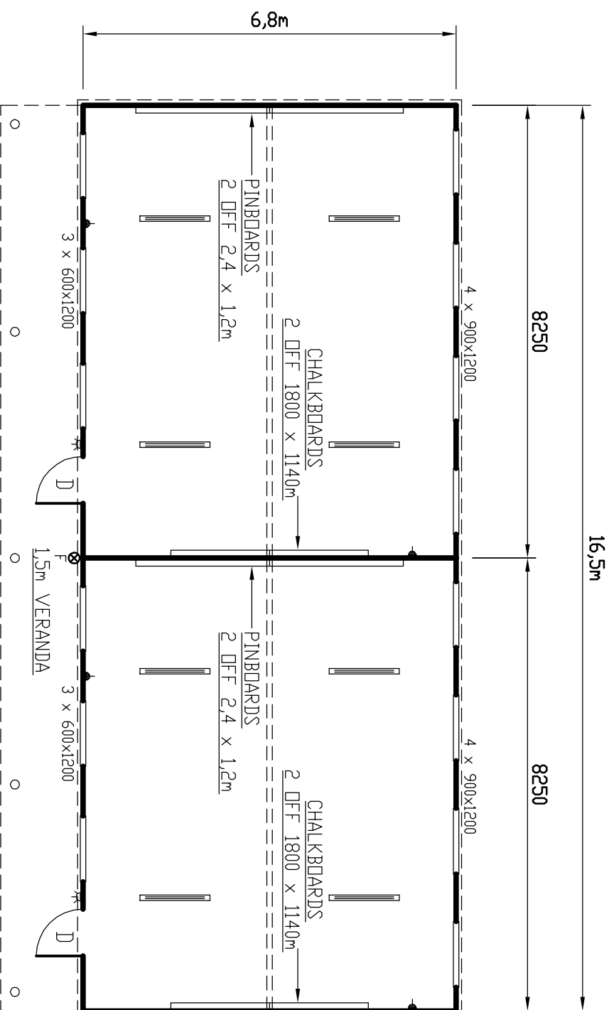
PLAN 112,2m 2
