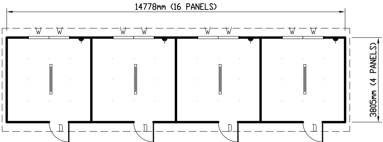
PLAN 56m 2
