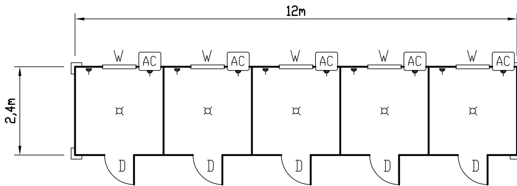
PLAN 28,8m 2
